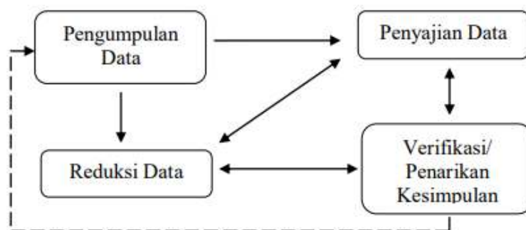
Gambar 3.1 Diagram Analisis Data
